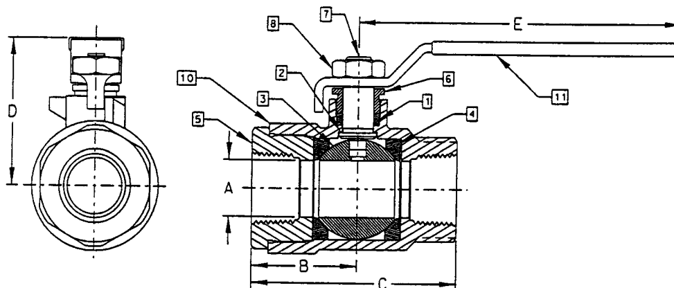
STAINLESS STEEL FULL PORT BALL VALVE
