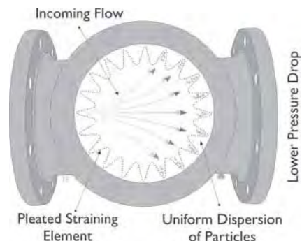
Figure 9: Top View - Basket Strainer - Pleated Straining Element
