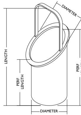
Figure 4: STYLE 'B' Slanted Type Basket Typically used for larger sized Simplex and Duplex Basket Strainers. Slanted inlet side reduces pressure drop across the strainer. Strainer cover presses down on handle to ensure straining element remains securely seated.
