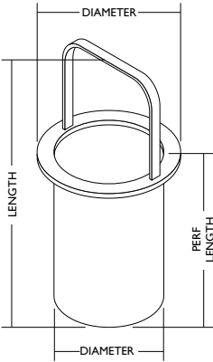
Figure 5: STYLE 'C' Basket Type Typically used for smaller sized Simplex and Duplex Basket Strainers. Strainer cover presses down on handle to ensure straining element remains securely seated.
